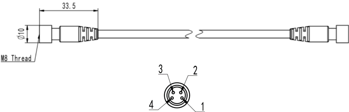
4-socket M8 Plug
